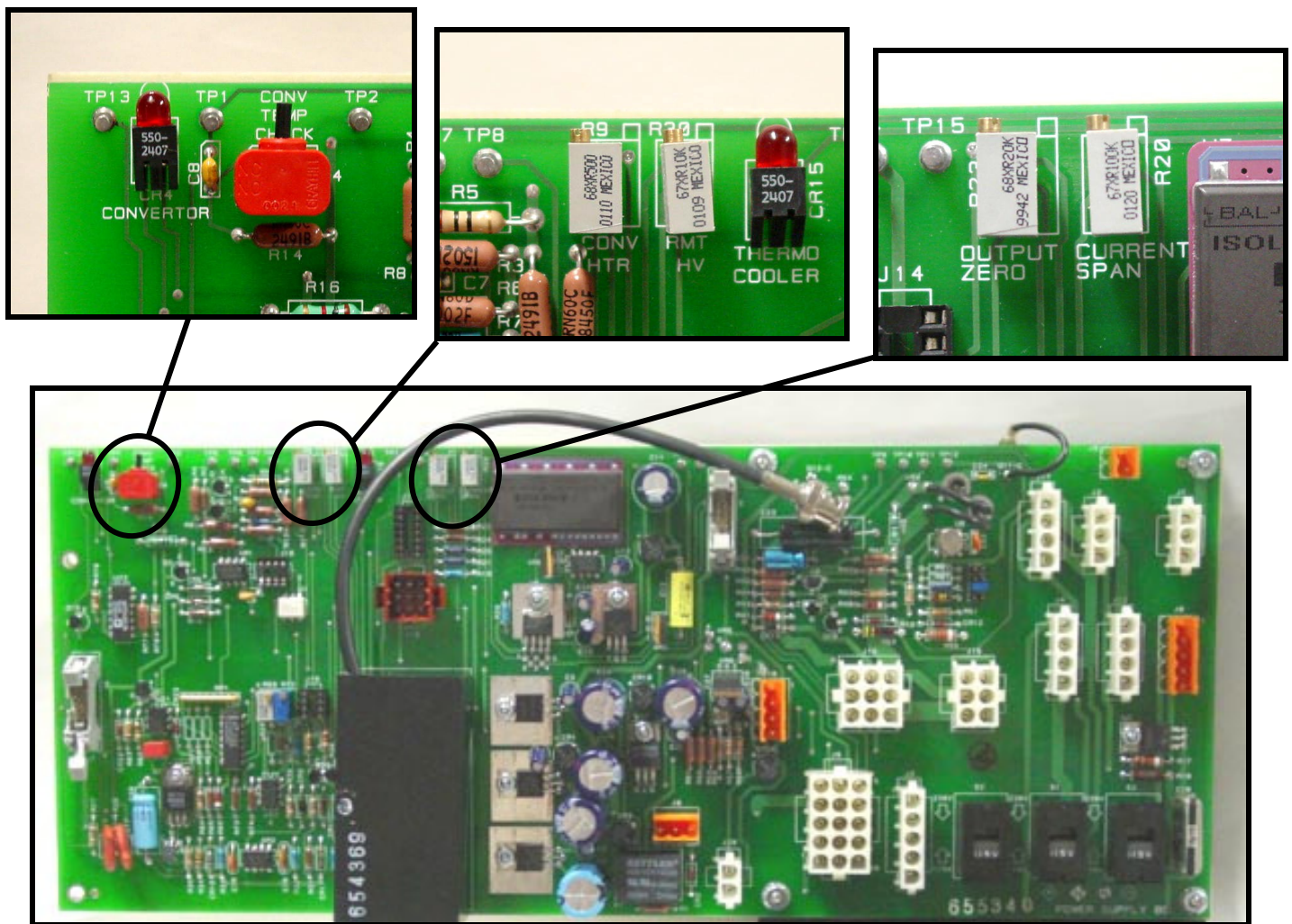
Figure 3-9. Power Supply Board
